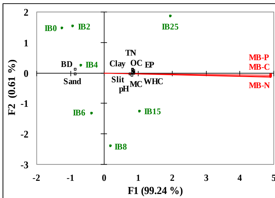
Figure 2. Redundancy analysis among seven iron mine overburden spoil ( IB_0 \rightarrow IB_{25} ) as well as nearby NF soil revealed the highest absolute scores on each of the first two axes of biological interest with site codes.
